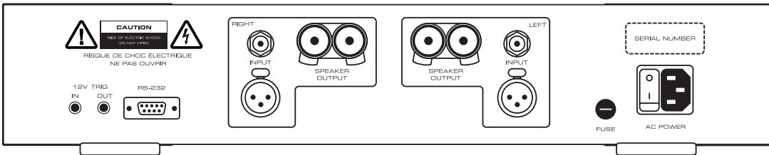
Figure 1: 330A Backpanel
