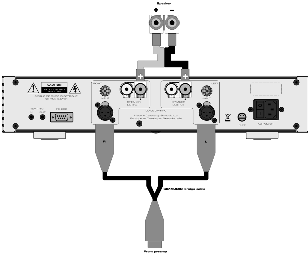
Figure 3: Bridged-Mono operation of the MOON 330A Power Amplifier
