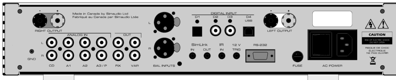
Figure 4: MOON 340i X Rear panel
