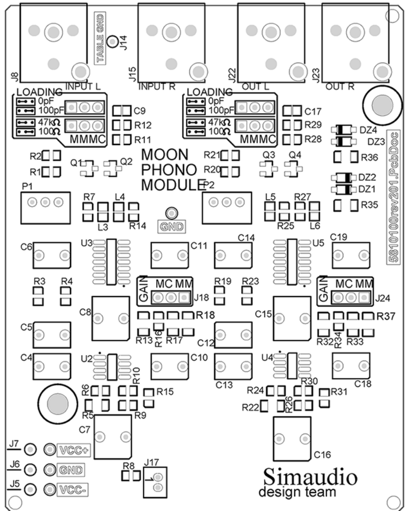
Figure 3: MOON 340i X Optional Phono Section Circuit Board Layout
